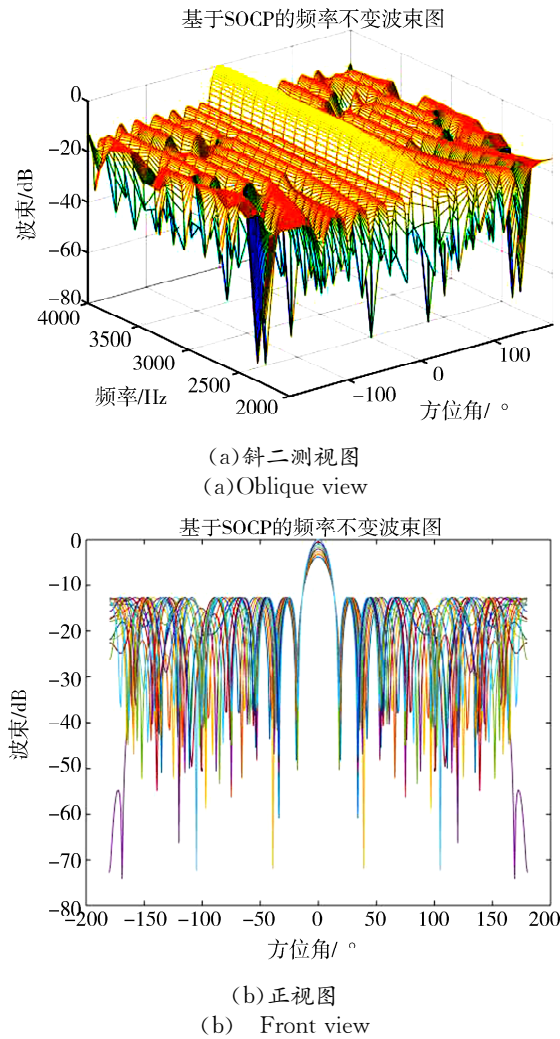
图 3 30 基于 SOCP 的频率不变波束图 Fig. 3 Frequency-invariant beam based on SOCP
