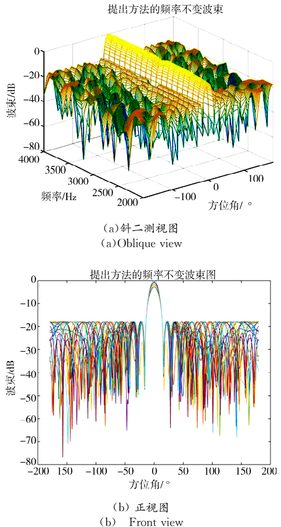
图 4 采用提出方法的频率不变波束图 Fig. 4 Frequency-invariant beam with proposed method
