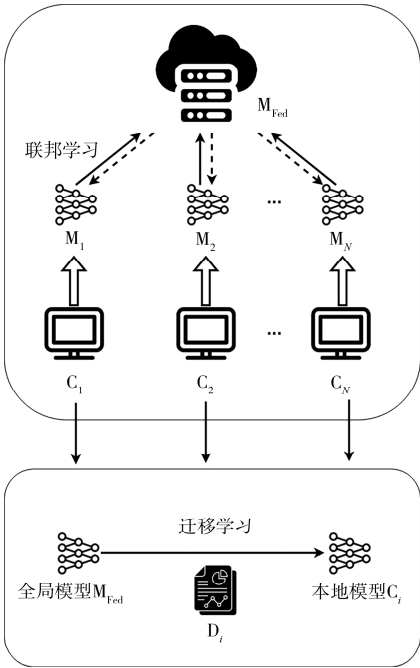
图 1 基于联邦迁移学习的日志异常检测框架 Fig. 1 Log anomaly detection framework based on federated transfer learning
